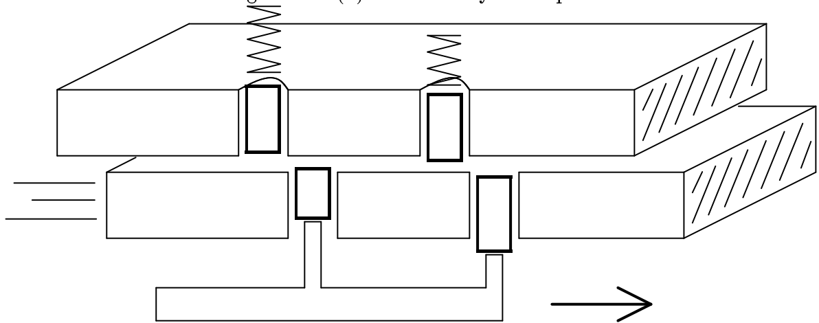
Figure 3.3: (b) Proper key allows plates to slide
