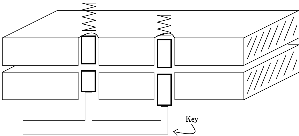
Figure 3.2: (a) Flatland key raises pins
