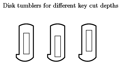
Figure 9.10: Workings of a disk tumbler lock
