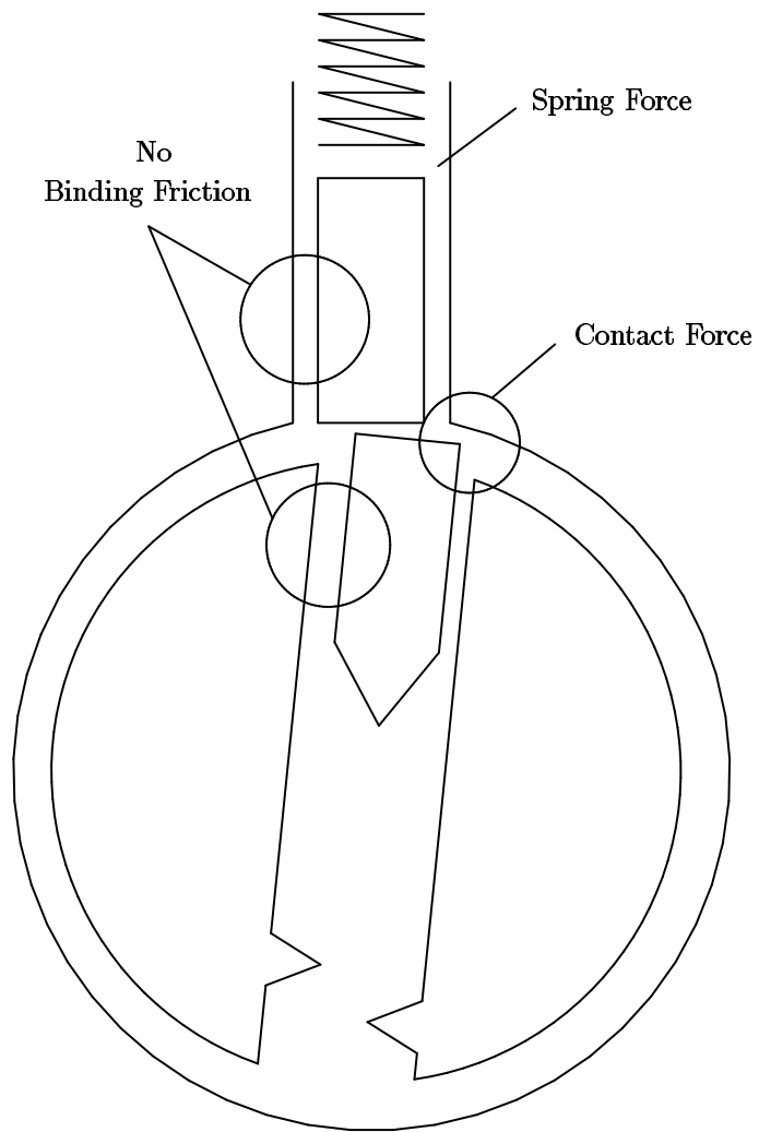
Figure 5.3: Pins at the sheer line
